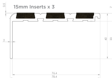
Profile TL77F
