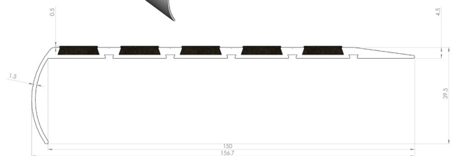
Profile TL150BR
