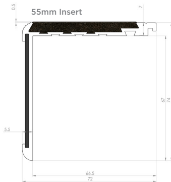
Profile TL55F
